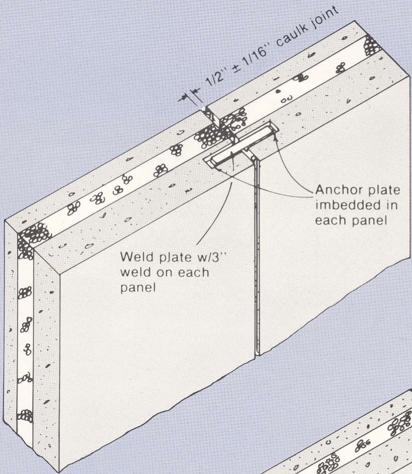
TOP CONNECTION
