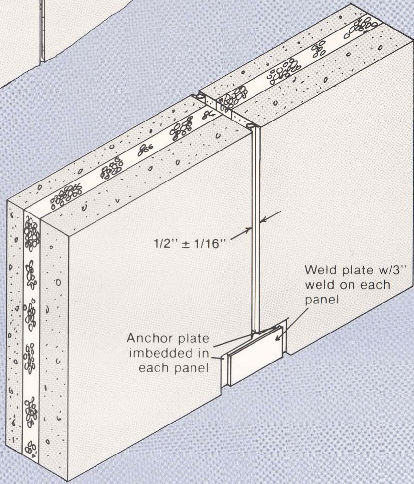
WALL CONNECTION
