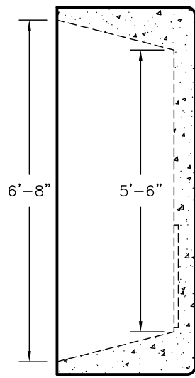
END VIEW
