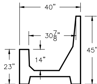
40" END VIEW
