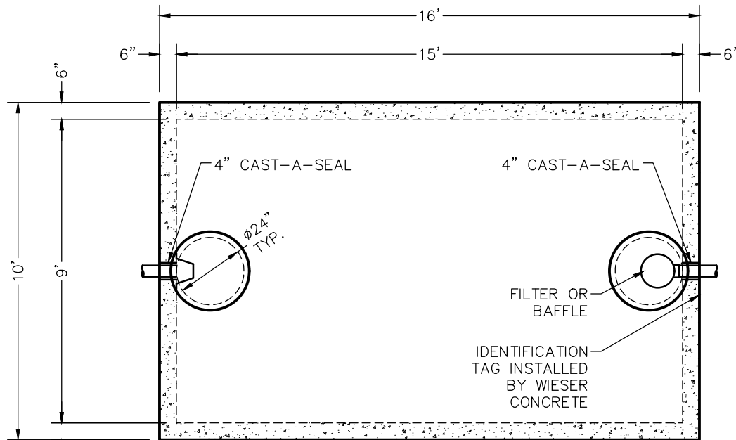
TOP VIEW
