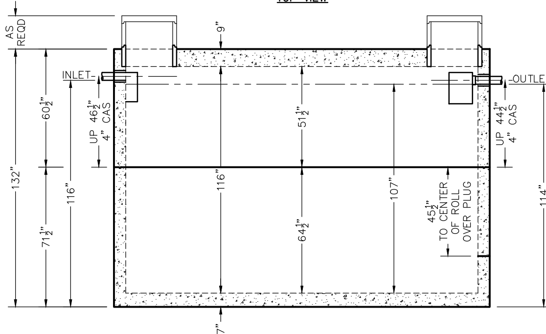
SIDE VIEW
