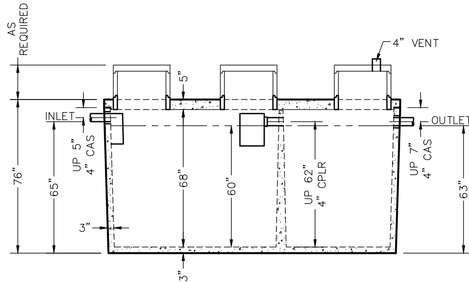
SIDE VIEW
