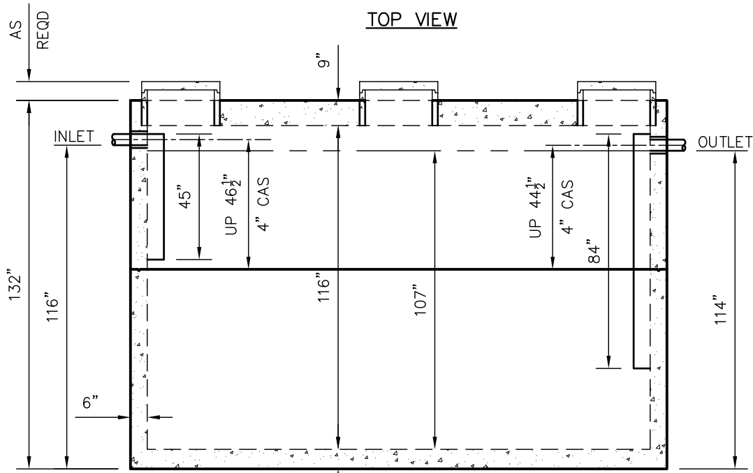
SIDE VIEW
