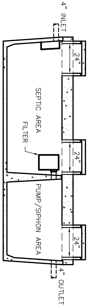
COMBINATION TANK
