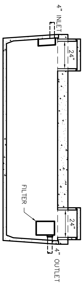
SEPTIC TANK
